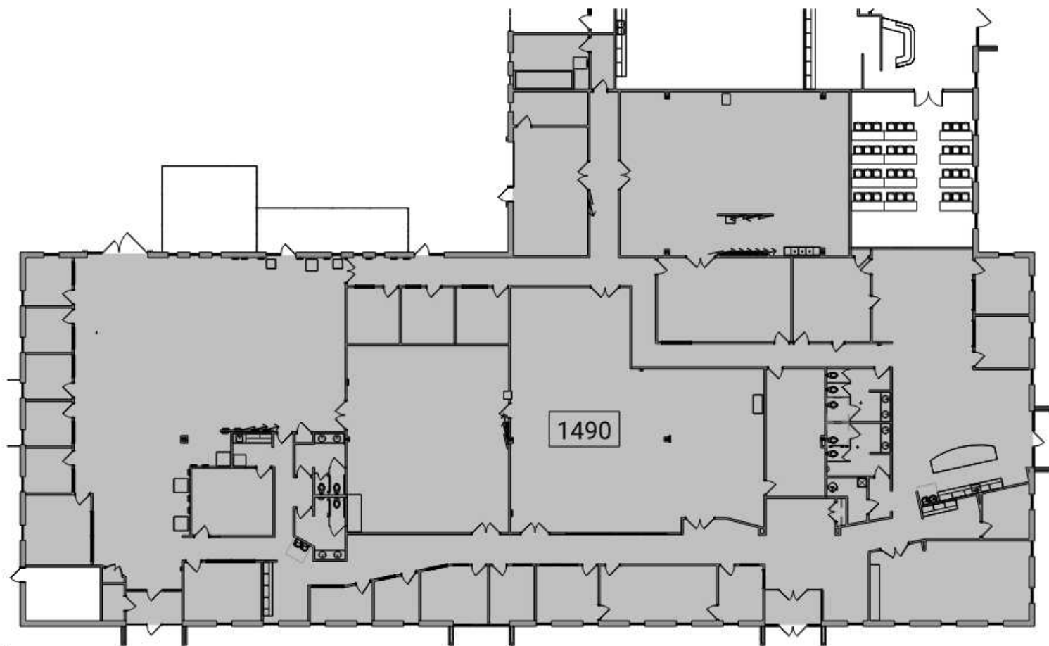
N 2 Suite 1490 - Existing Floor Plan LA-90 4' 8' 16' 1" = 30'-0"
