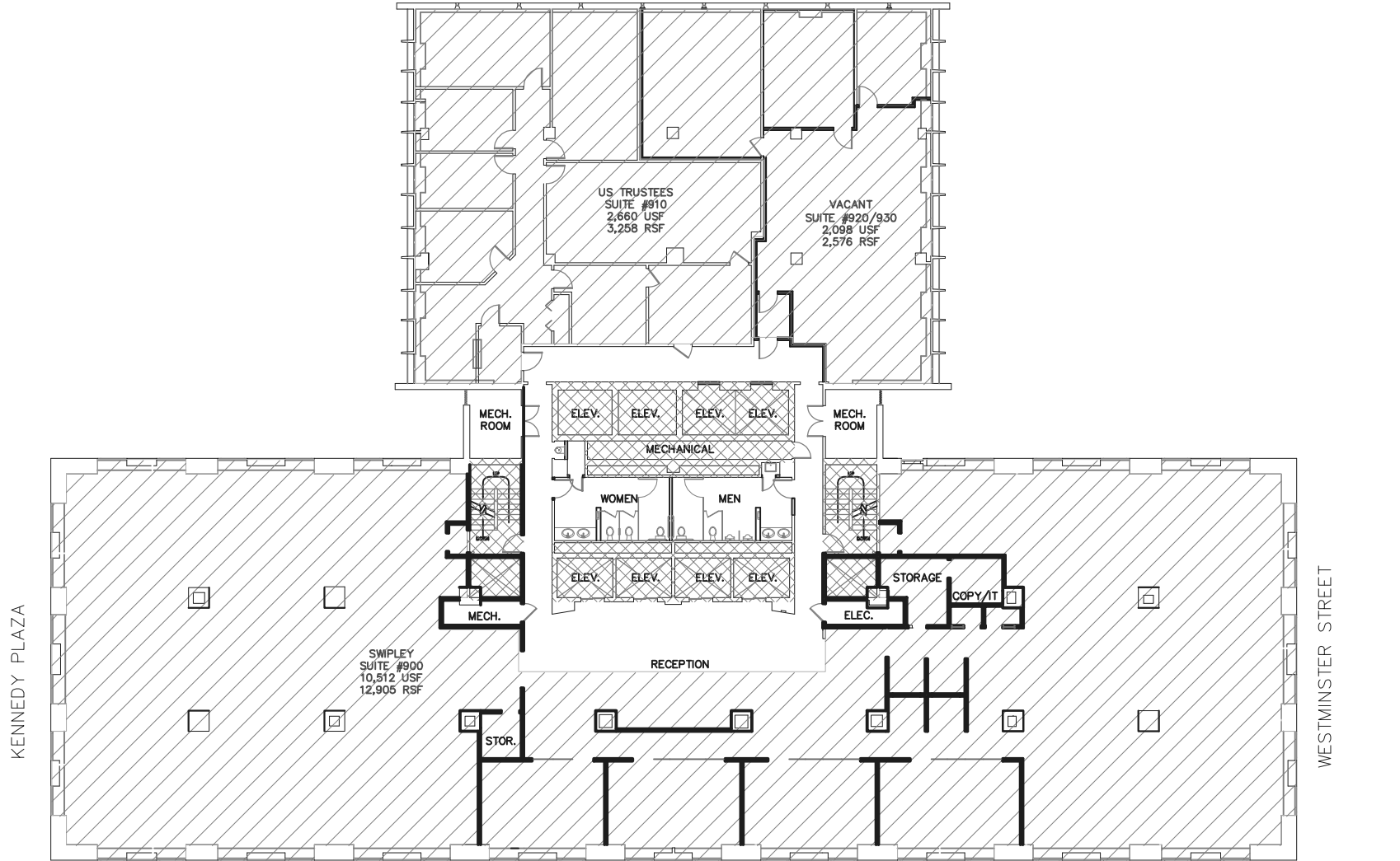
NINTH FLOOR PLAN
