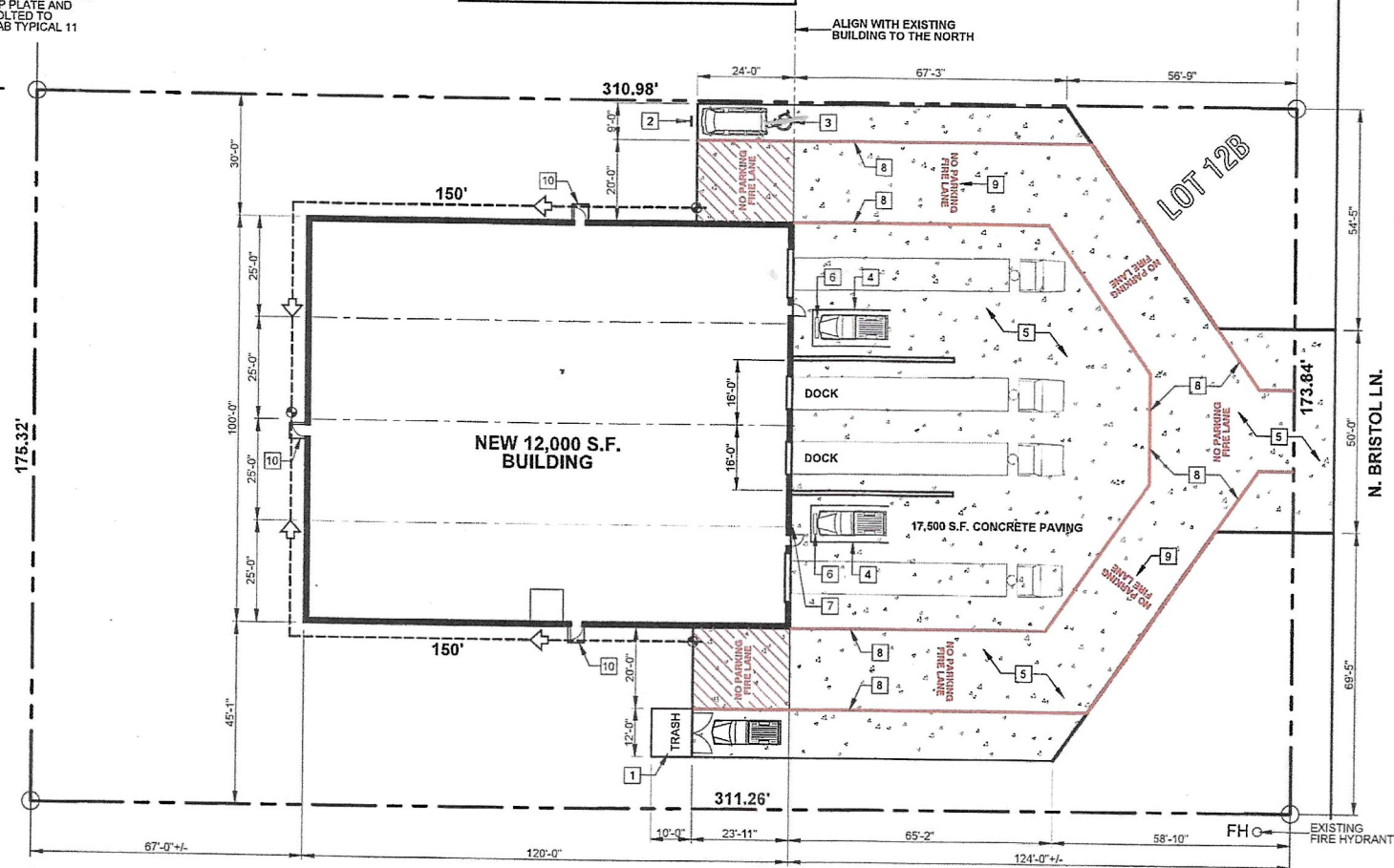
S I T E P L A N 1"=20' 4 CAR PARKING
