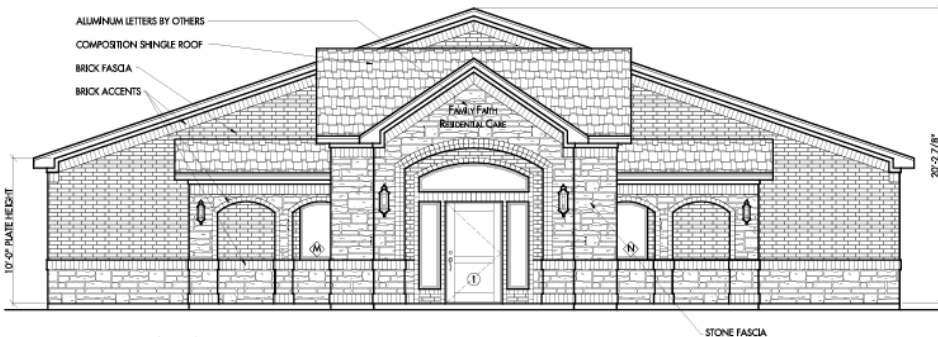
SOUTH ELEVATION
