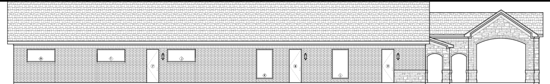
WEST ELEVATION
