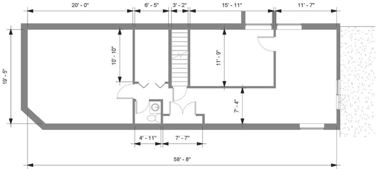
① LOWER LEVEL FLOOR PLAN 1/8" = 1'-0" 1,400 SF
