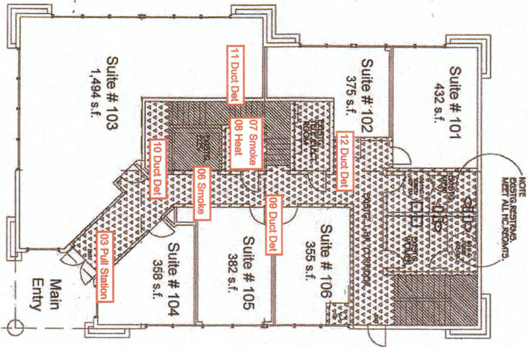
First Floor
