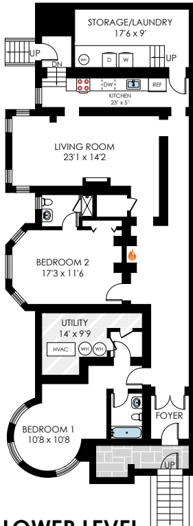
LOWER LEVEL 1788 FIN. SQ. FT. 99 UNFIN. SQ. FT. 7'6" CEILING
