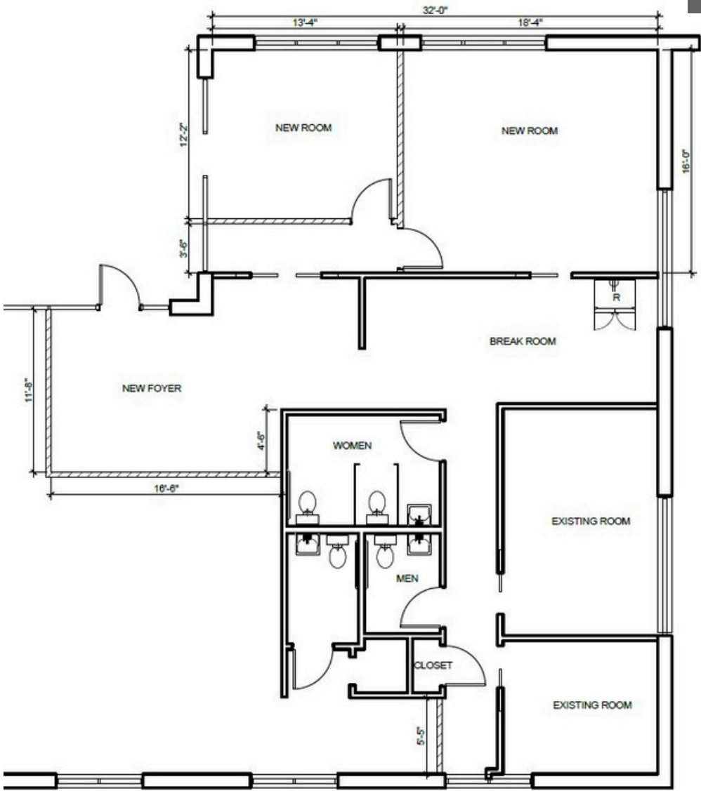
Floor Plan
