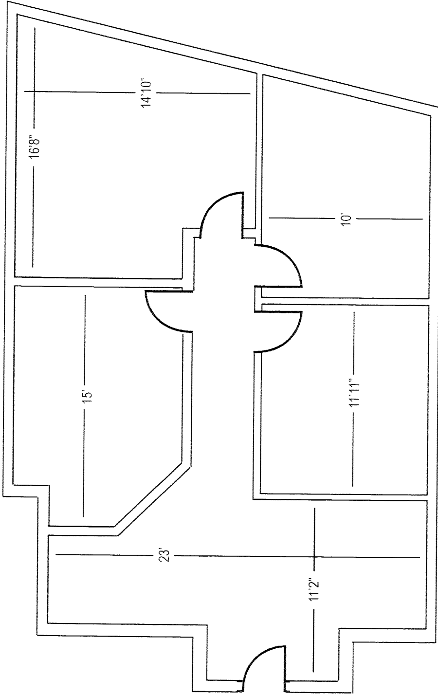
Suite 214 Floor Plan - 1,158 SF
