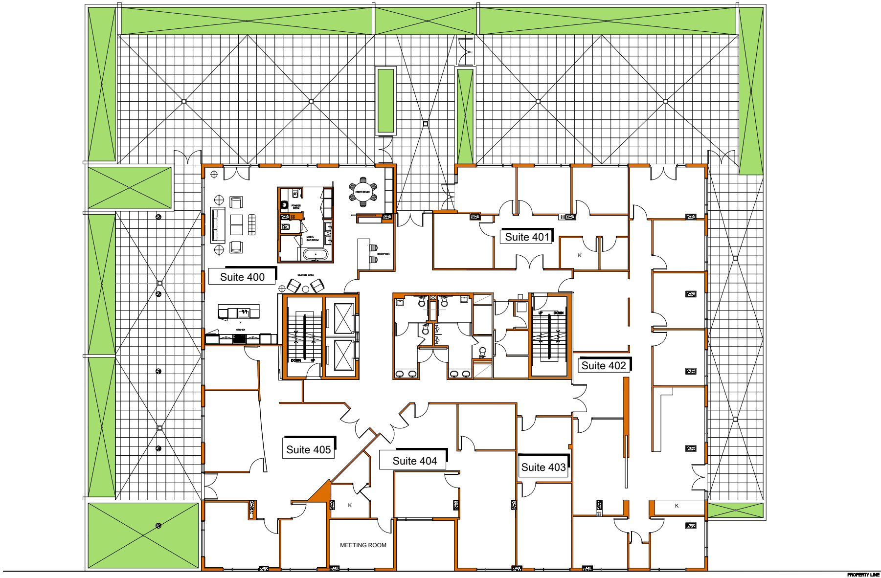
4TH-FLOOR-PLAN-OFFICE UPDATE 17-11-2016
