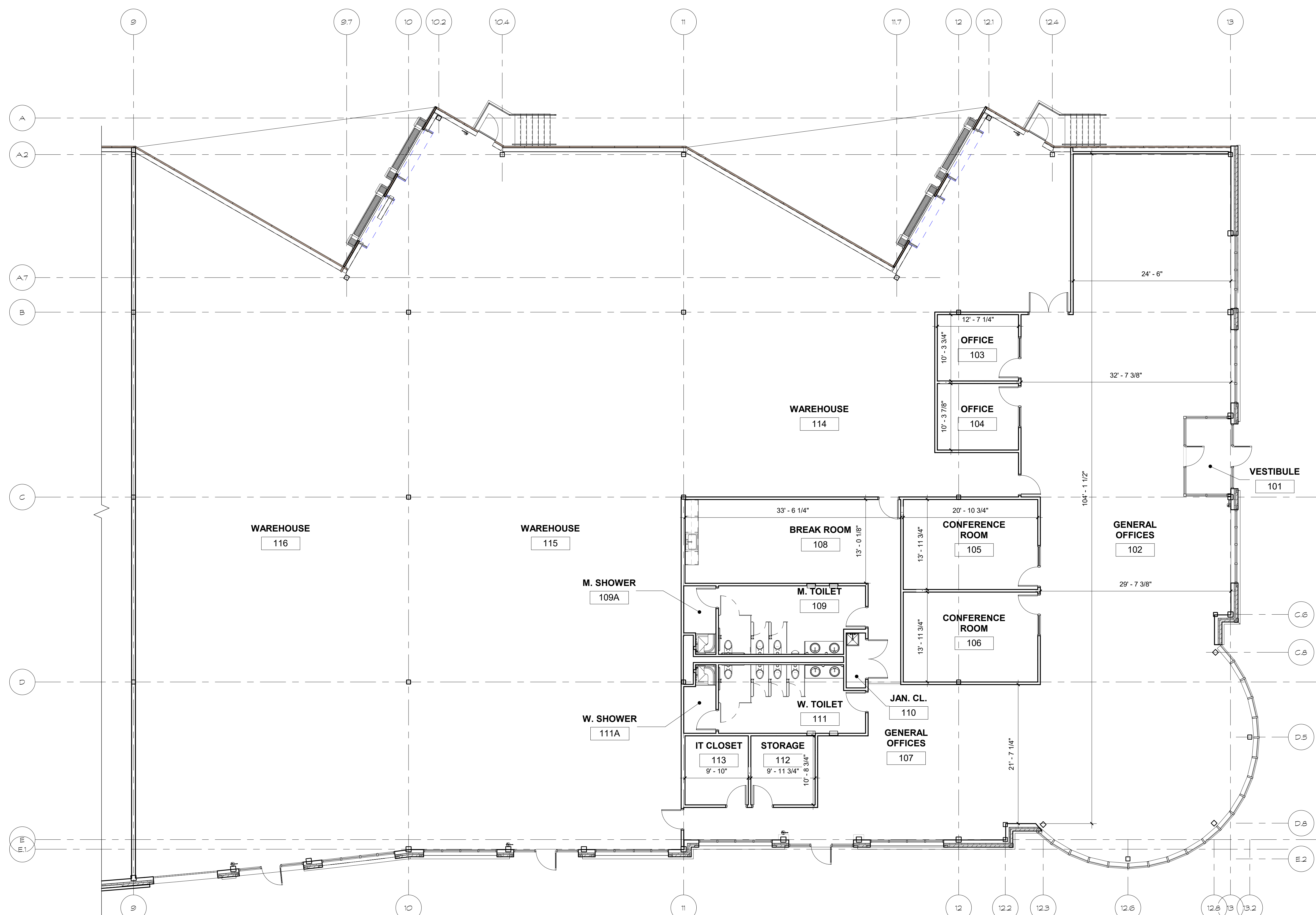
1 Tenant Space Overall Plan 1/8" = 1'-0"
