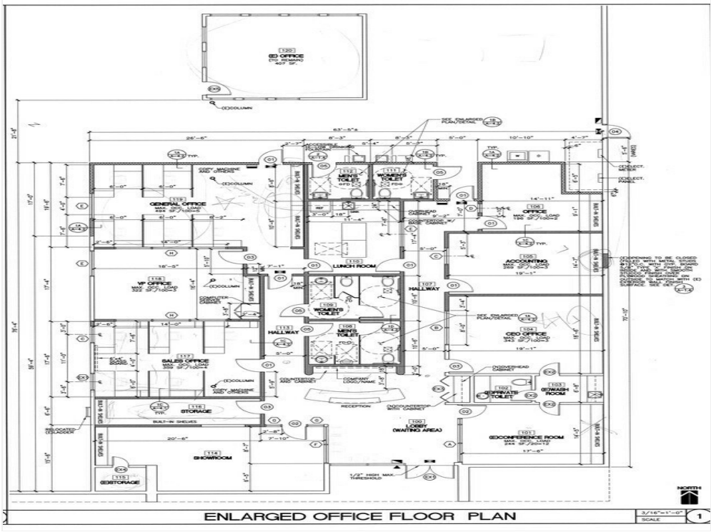
Office Plan
