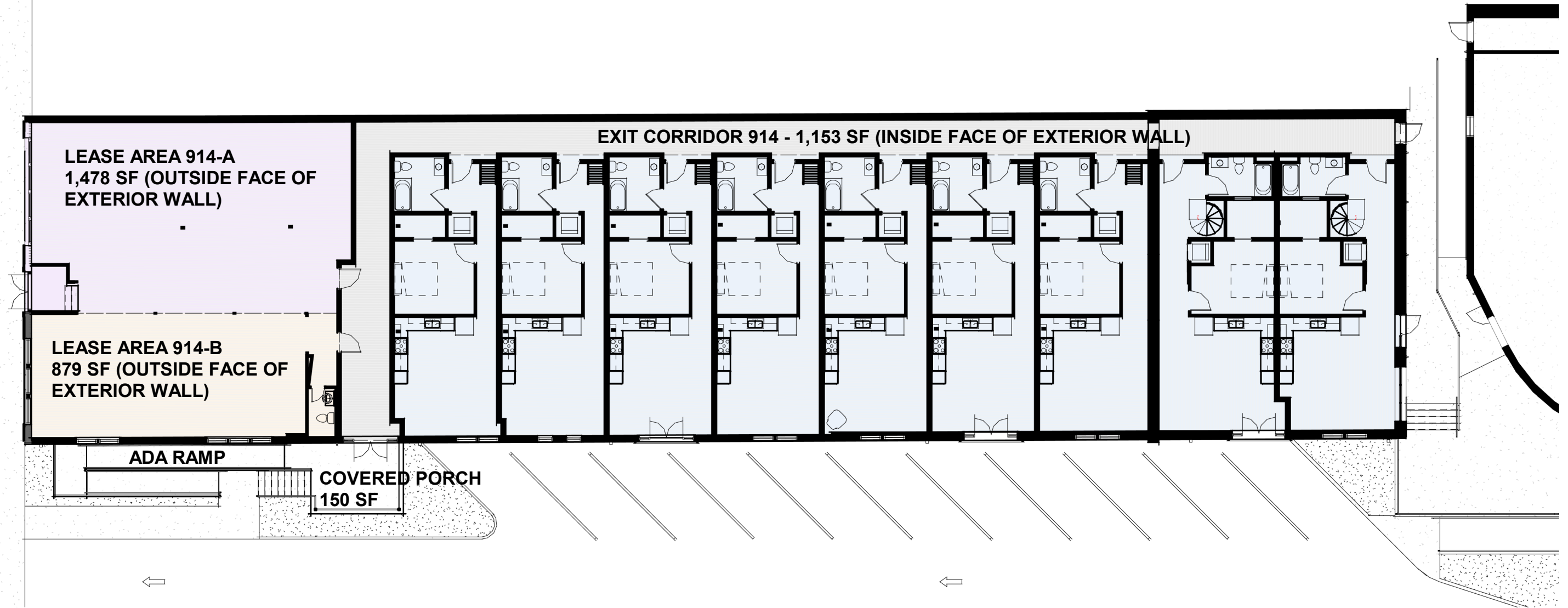
1 FIRST FLOOR - 914 LADY LEASE AREA PLAN 1/16" = 1'-0"
