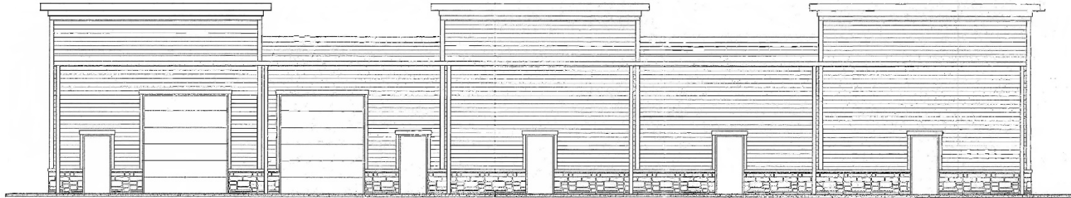
REAR ELEVATION
