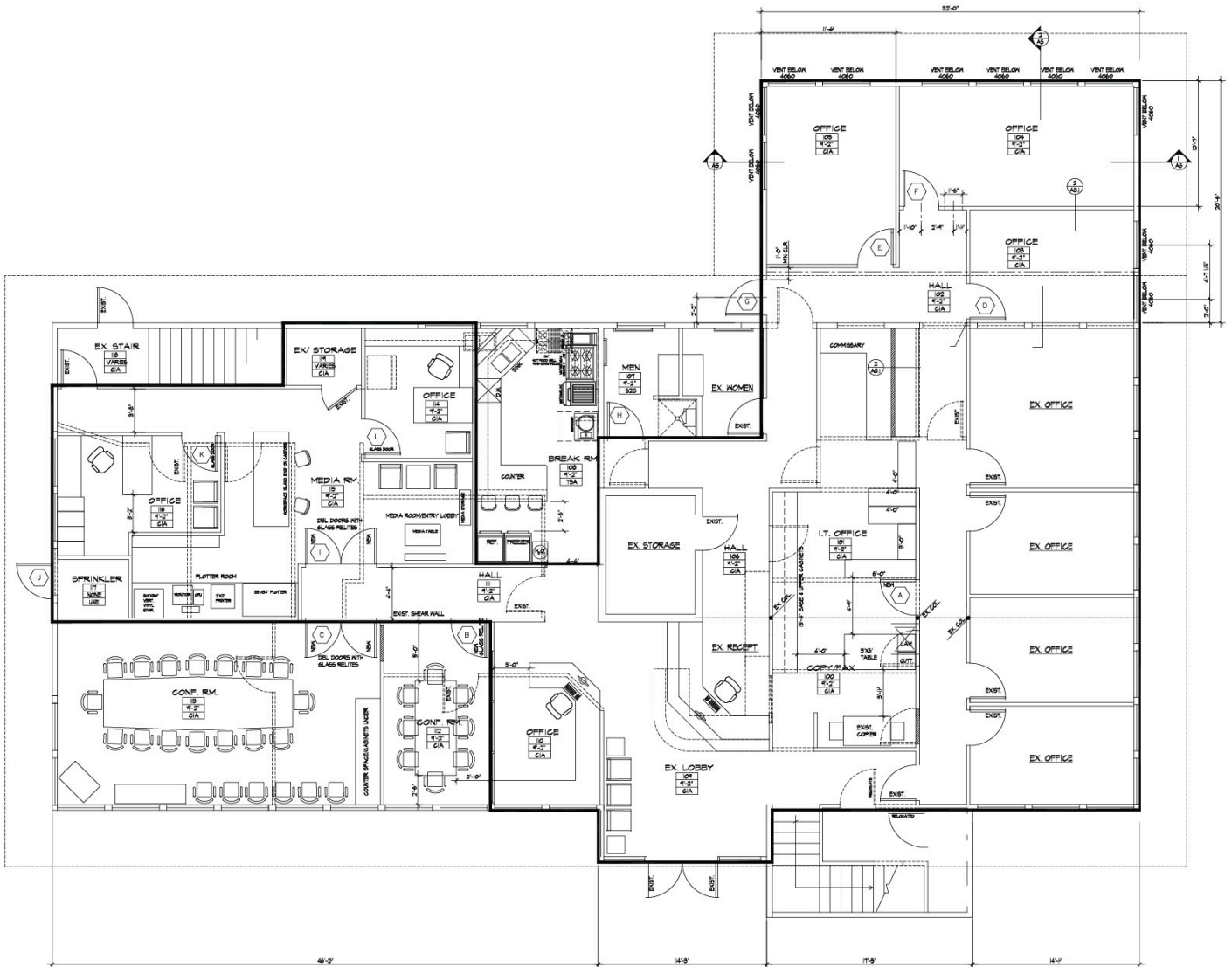
FIRST FLOOR PLAN – MAIN OFFICE BUILDING W-1-0 3474 SF
