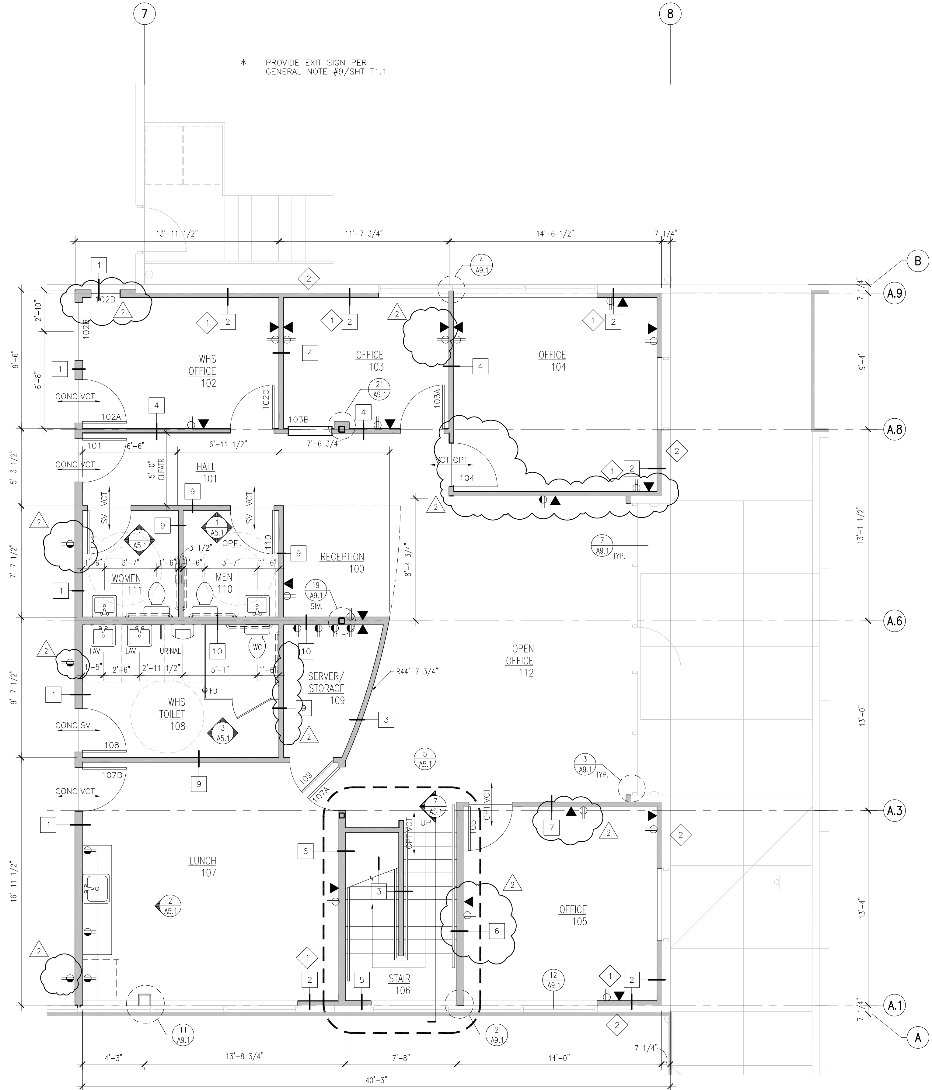
NORTH FIRST FLOOR PLAN SCALE: 1/4"=1'-0"
