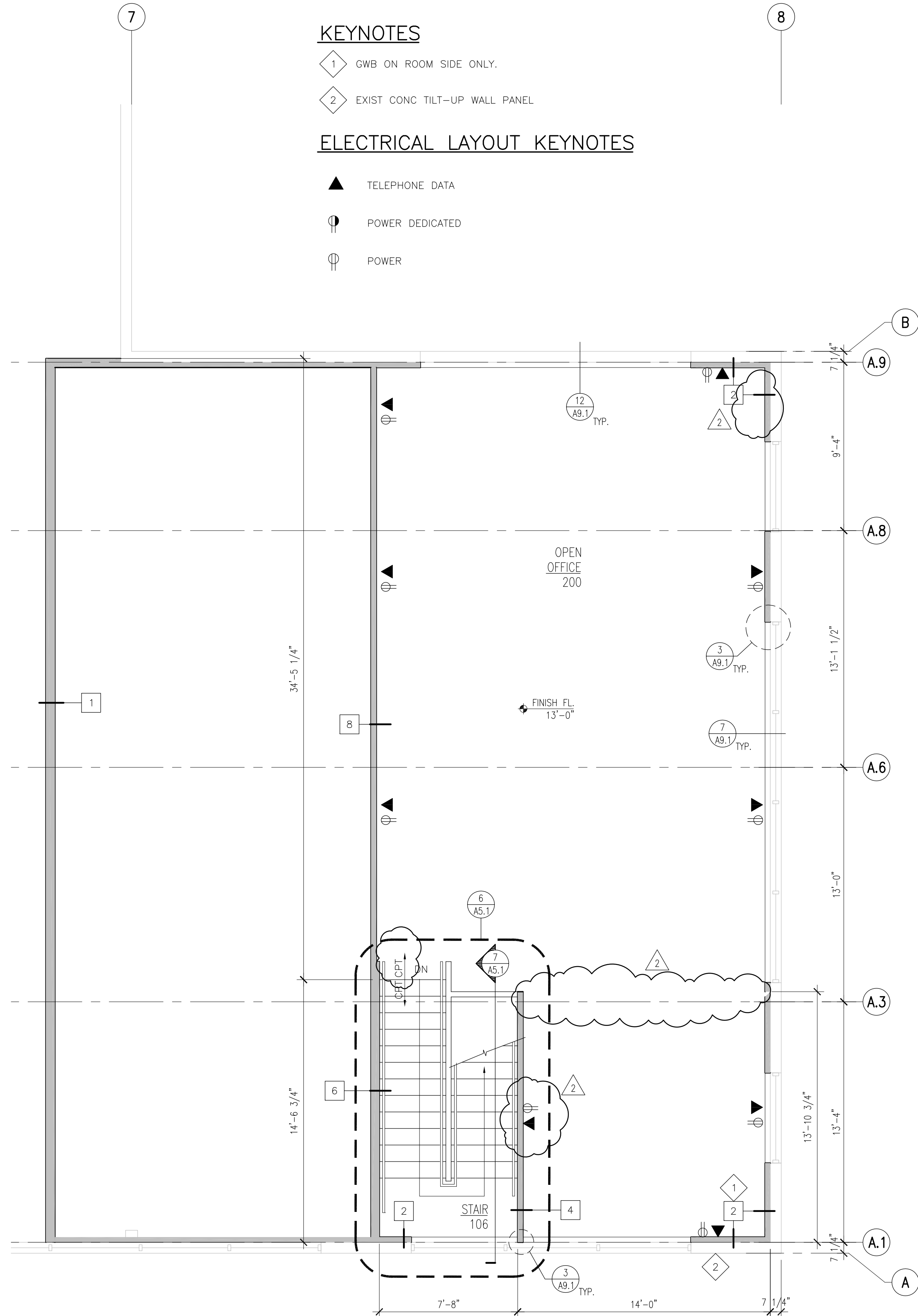
NORTH SECOND FLOOR PLAN SCALE: 1/4"=1'-0"
