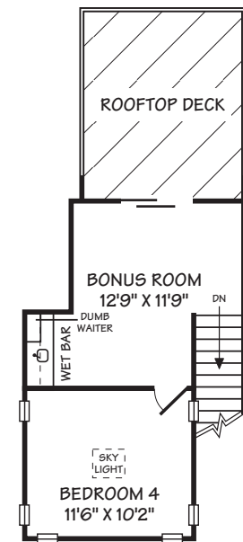
THIRD LEVEL 8'3" CEILING
