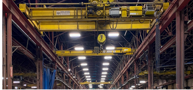
NORTH-SOUTH CRANE BAY: (2) 20 TON CRANES; (2) 5 TON CRANES
