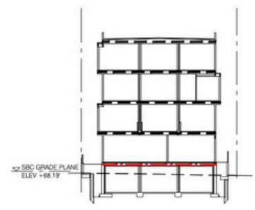
3 HORIZONTAL FIRE SEPARATION 1/16" = 1'-0"
