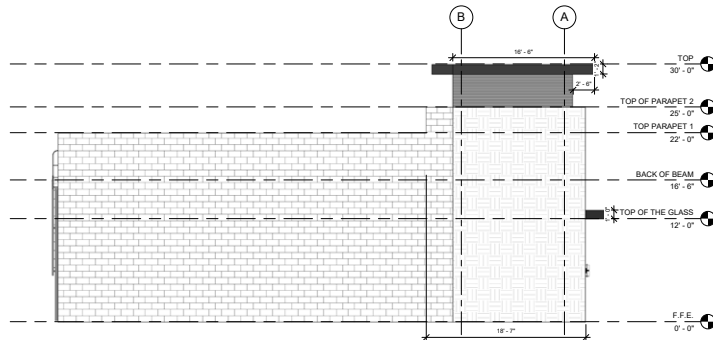
2 LEFT ELEV. 3/16" = 1'-0"
