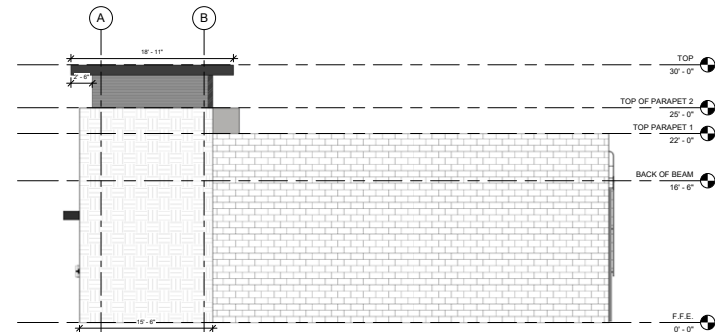
3 RIGHT ELEV. 3/16" = 1'-0"
