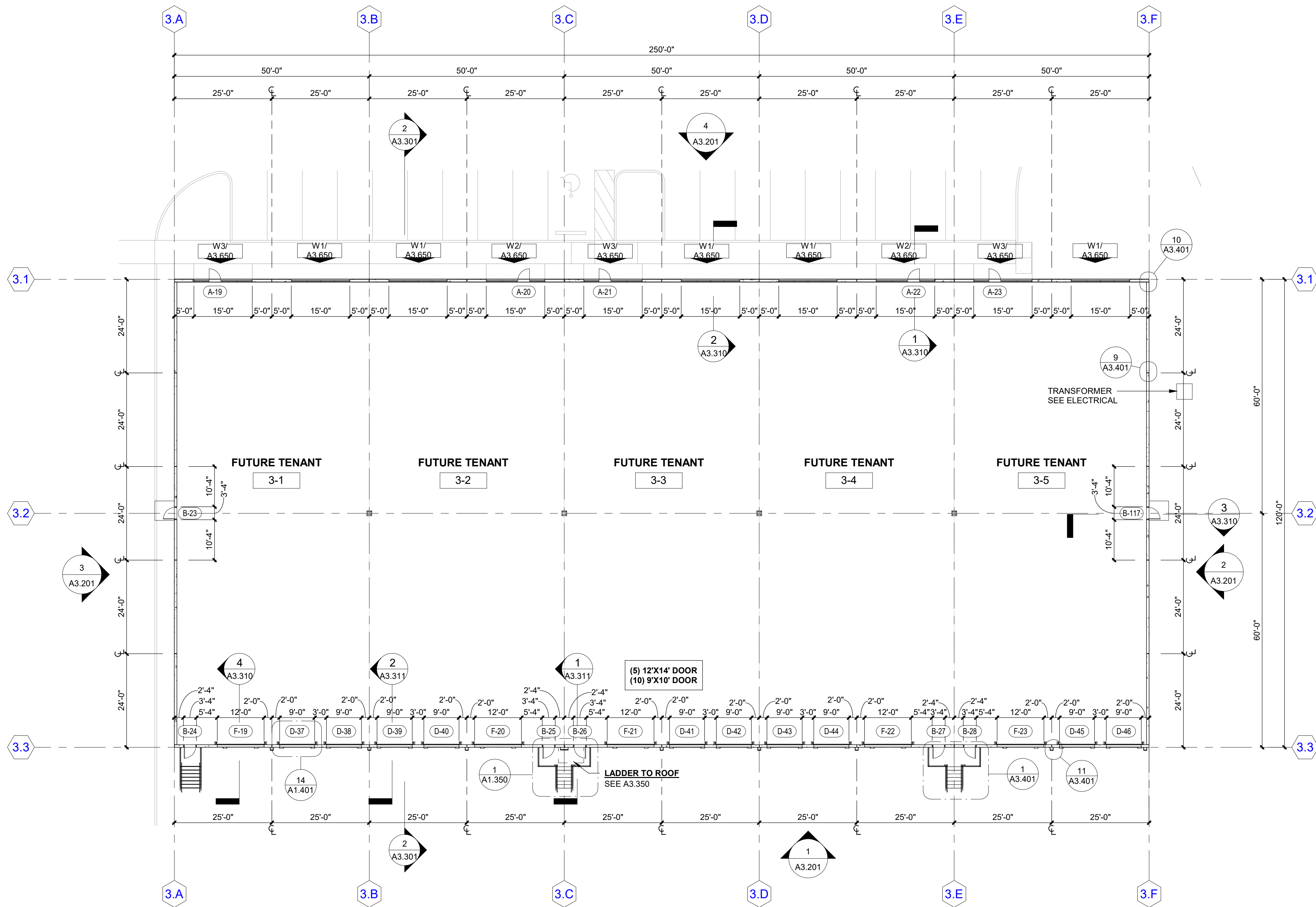
1 BUILDING 3 FLOOR PLAN A3.101 SCALE: 1/16" = 1'-0"
