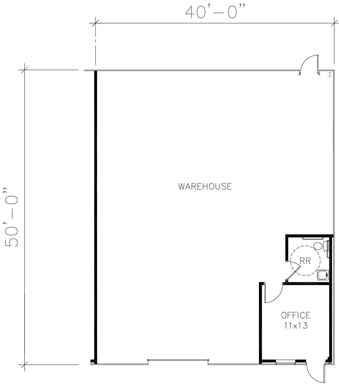
A FLOOR PLAN SCALE : 1/8" = 1'0"
