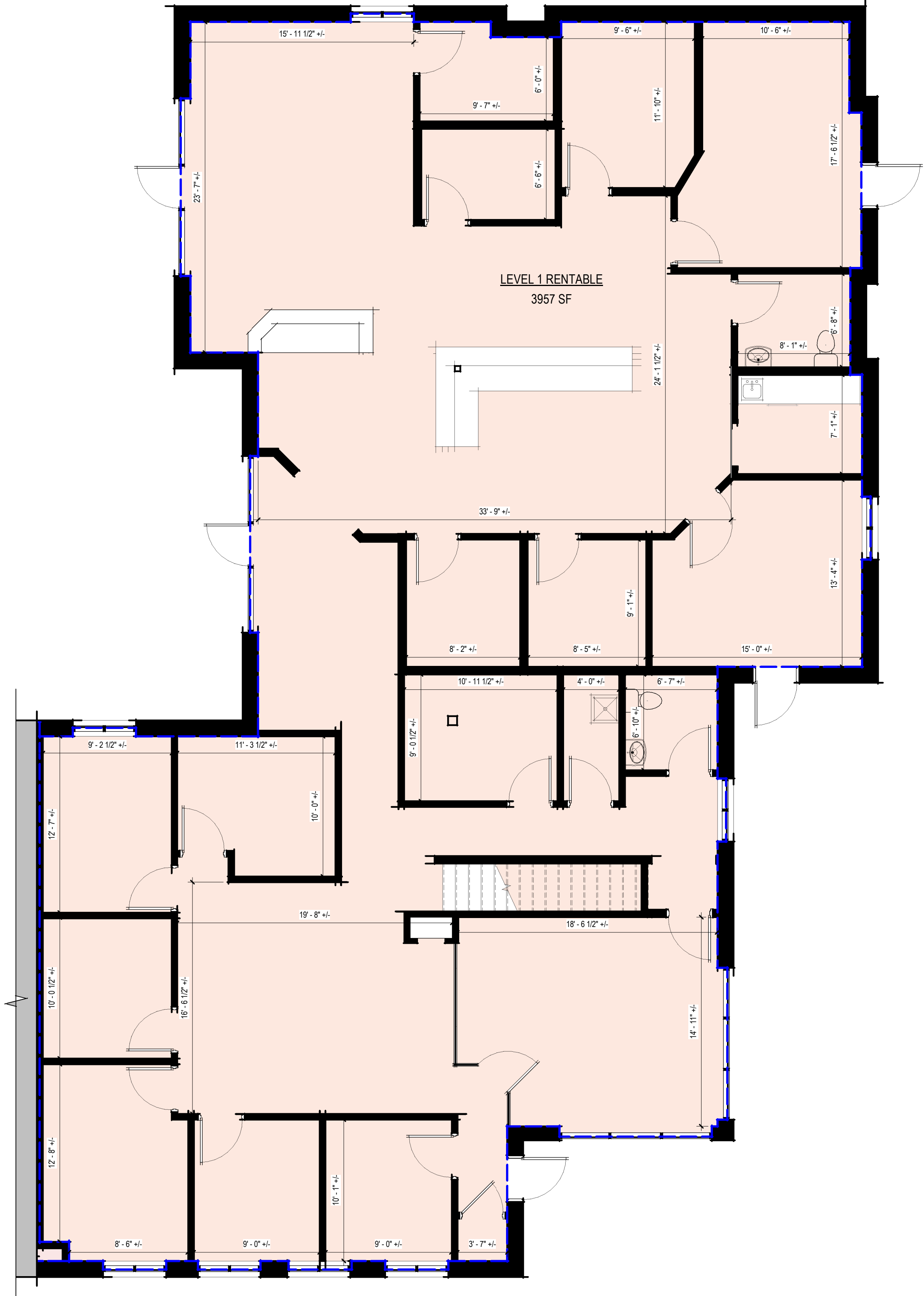
1 LEVEL 1 - RENTABLE AREA 3/16" = 1'-0"
