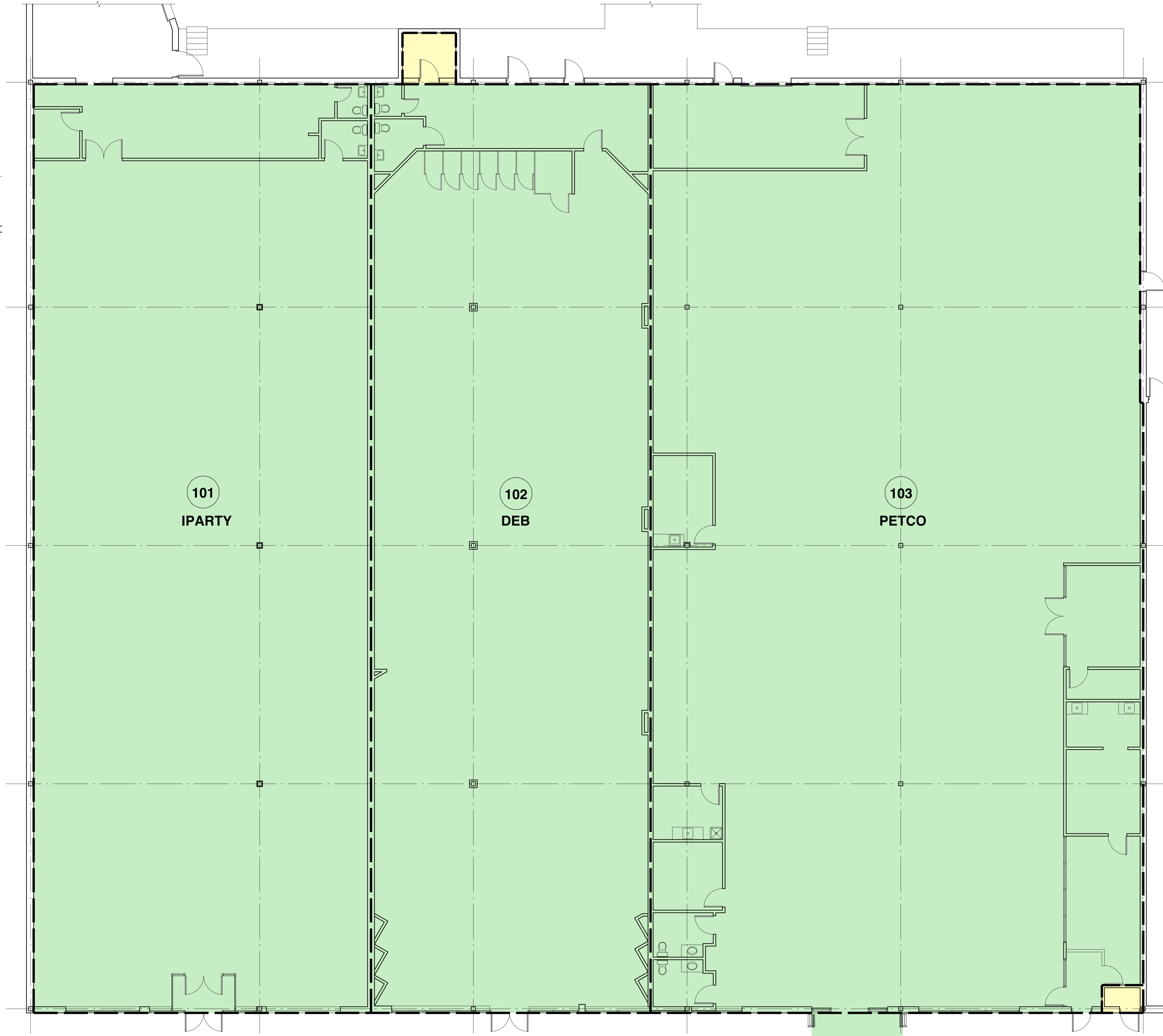
1 FIRST FLOOR PLAN SCALE: 1/8" = 1'-0" 2' 4' 8' 16'
