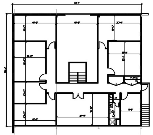
Mezzanine Plan
