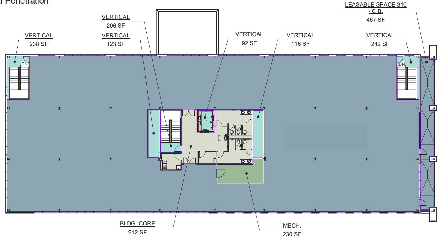
3 3RD FLOOR PLAN 1/16" = 1'-0"
