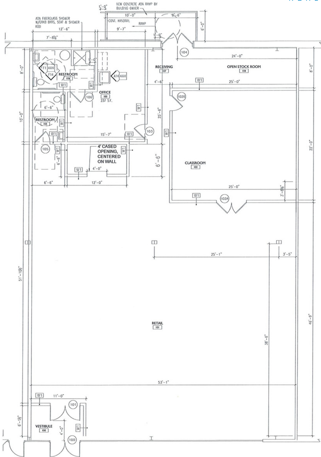
AI FIRST FLOOR PLAN
