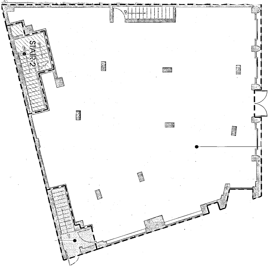
FLOOR PLANS: GROUND FLOOR - 2,510 SF
