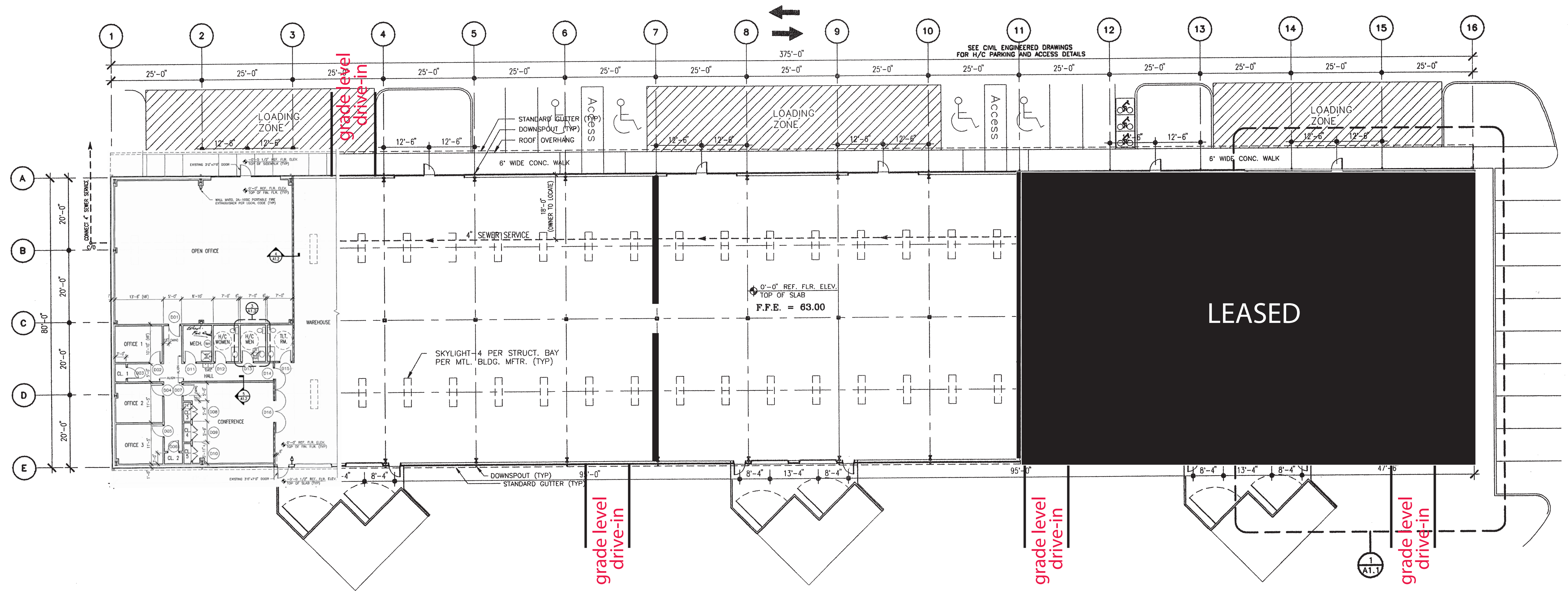
1 A1.0 BUILDING FLOOR PLAN 1/16" = 1'-0"
