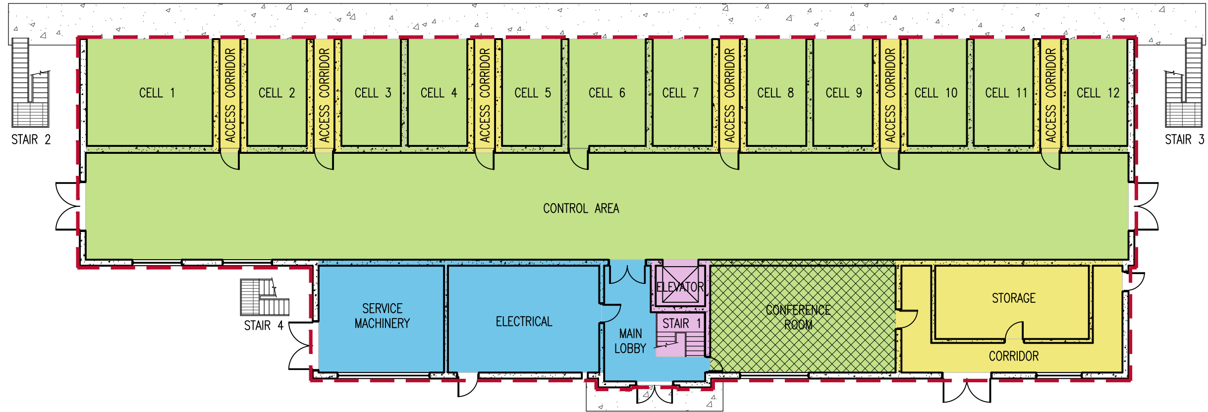
1 FIRST FLOOR PLAN SCALE: 1/16" = 1'-0"
