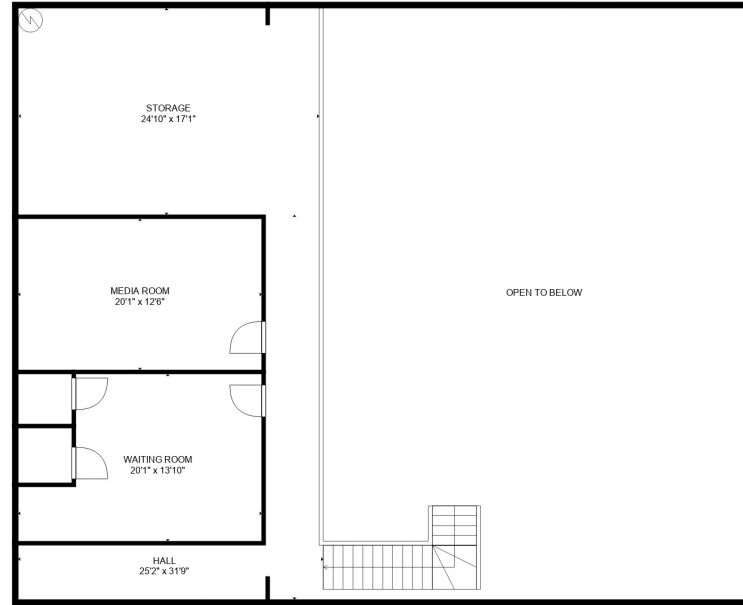
FLOOR 2
