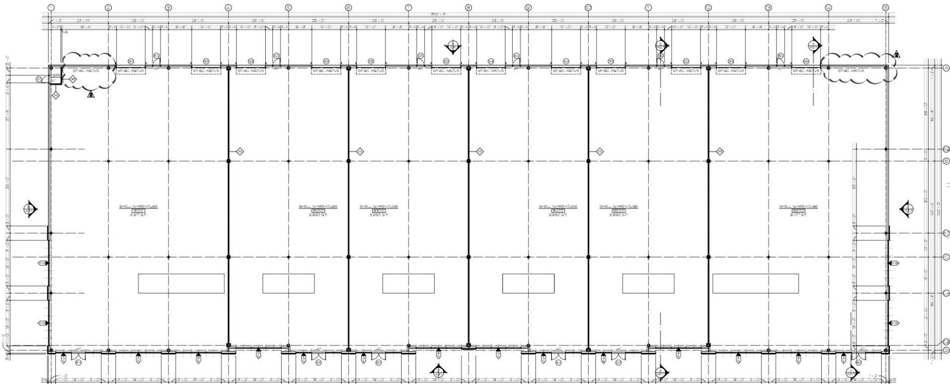
B1 OVERALL FLOOR PLAN - BUILDING B
