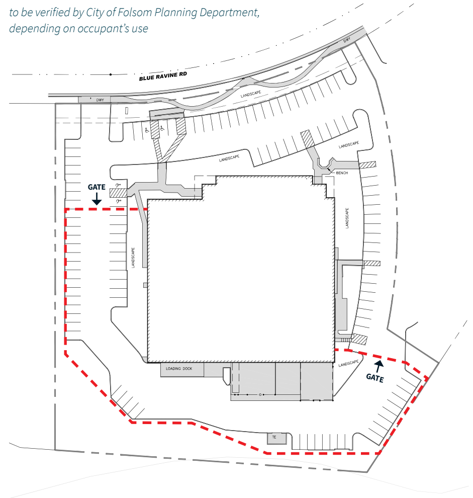
site plan with potential fence/gate
