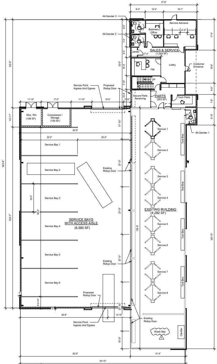
First Floor Plan 3/32" = 1'-0"
