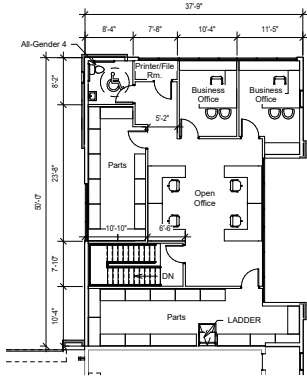
Second Floor Plan 3/32" = 1'-0"
