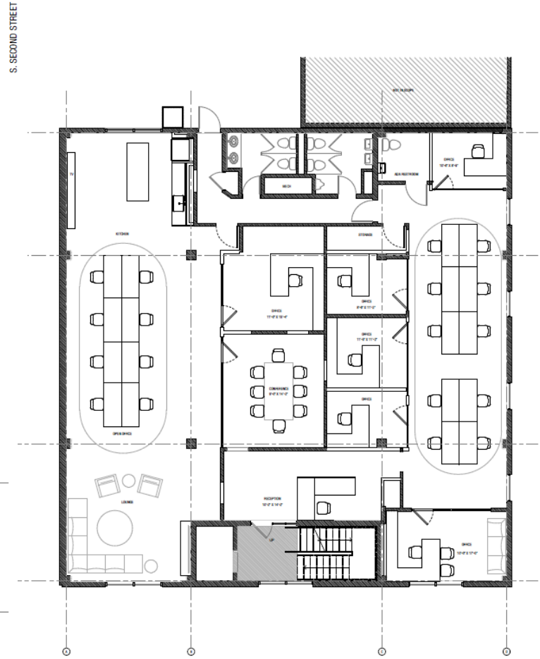
SECOND FLOOR 3,720 SF
