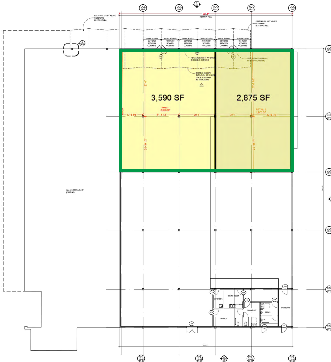
07 NEW CONSTRUCTION PLAN SCALE: 1/8" = 1'-0"
