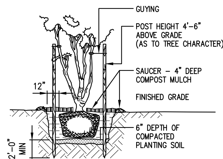
MULTI-TRUNK PLANTING DETAIL NOT TO SCALE
