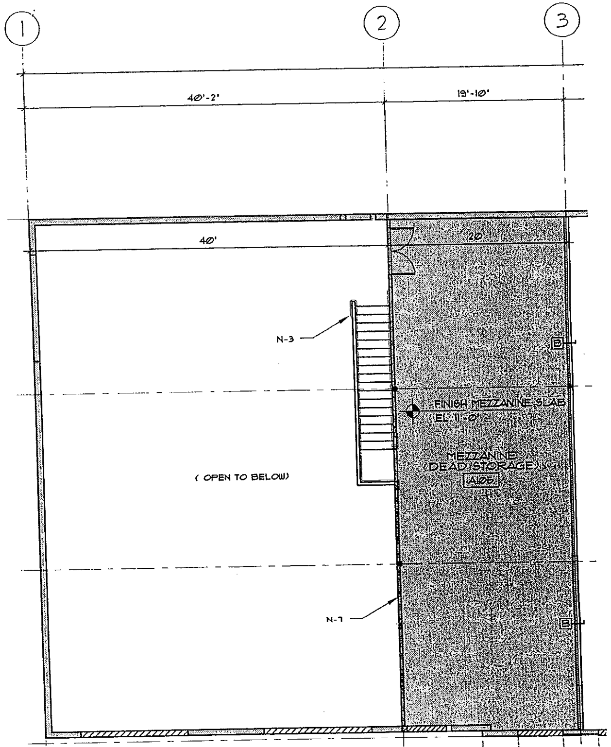
PLAN - LEVEL TWO
