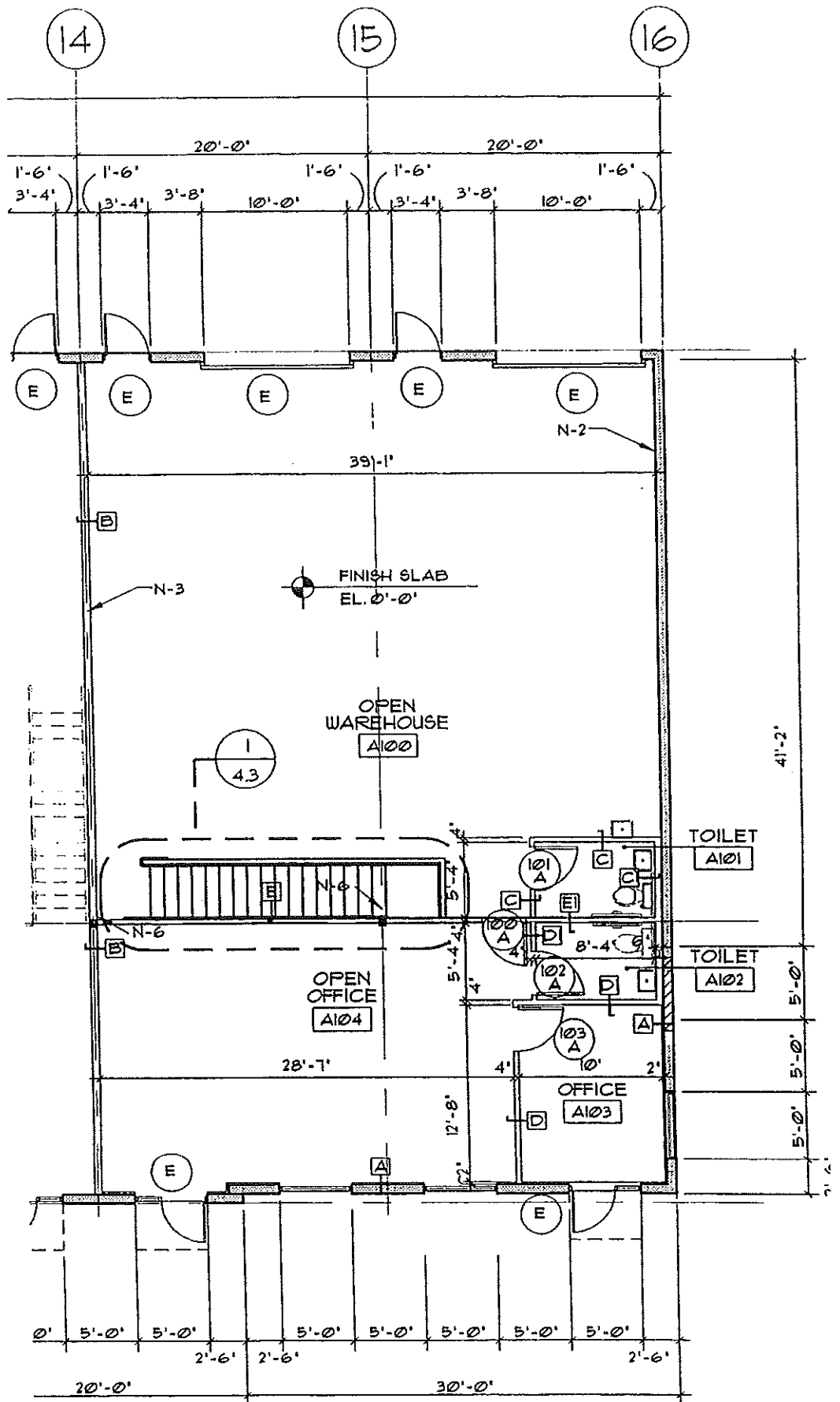
PLAN - LEVEL ONE
