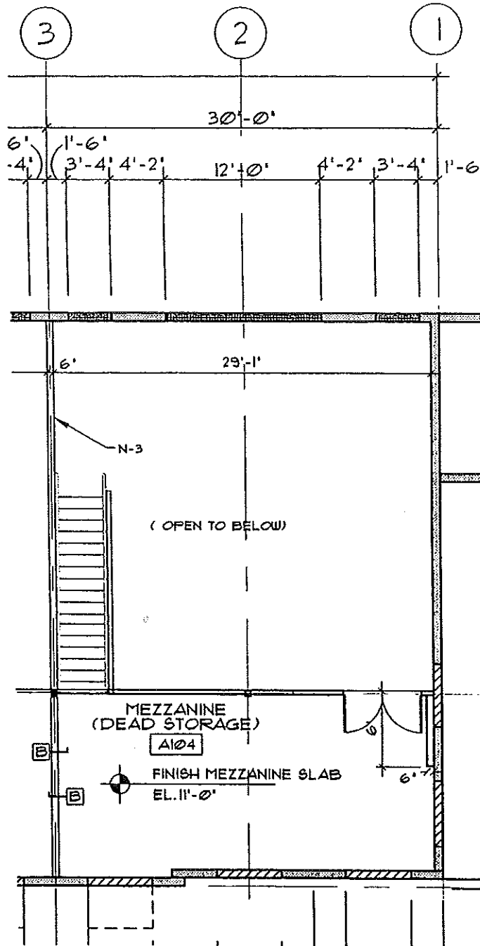
PLAN - LEVEL TWO
