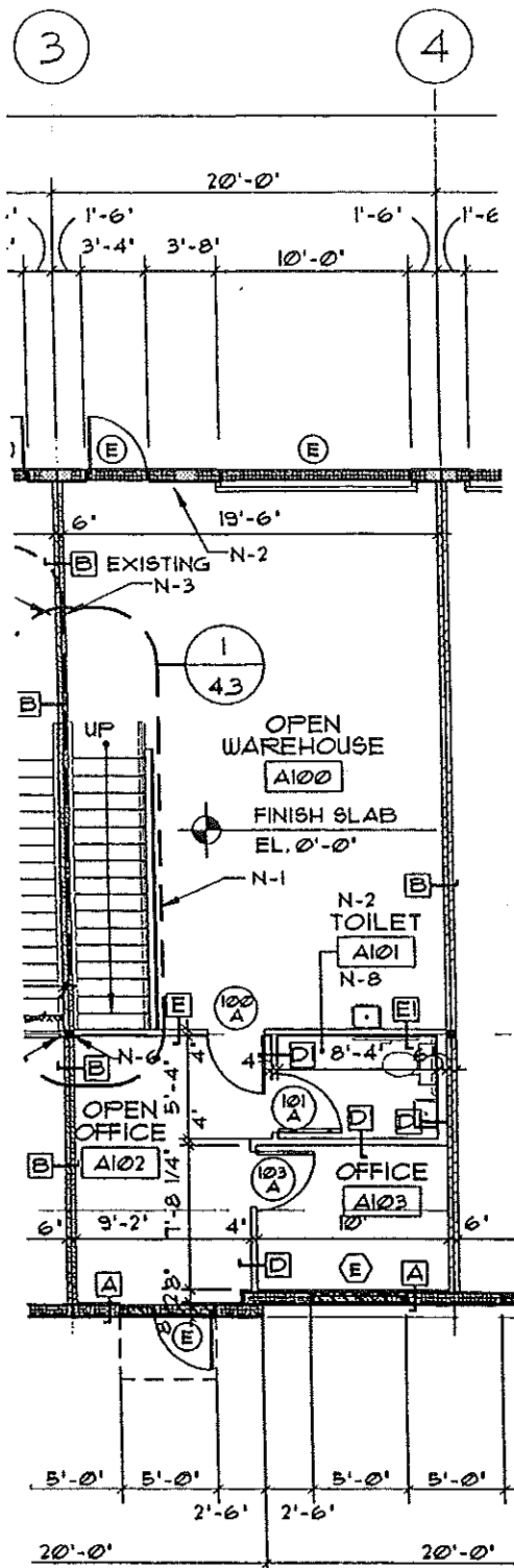
PLAN - LEVEL ONE
