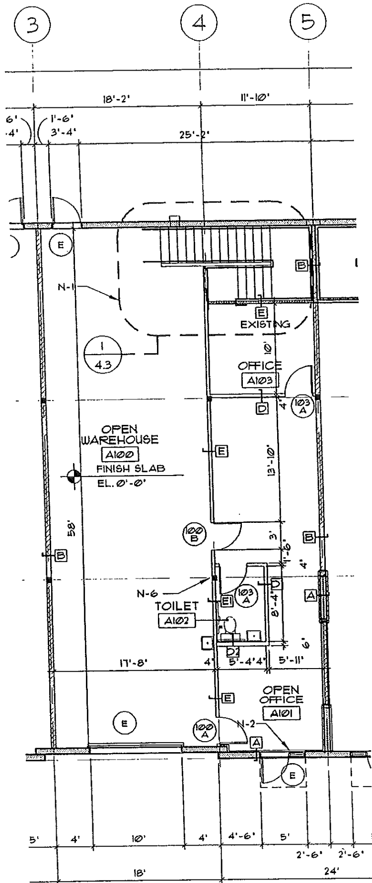
PLAN - LEVEL ONE
