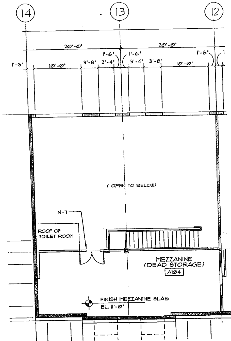
PLAN - LEVEL TWO
