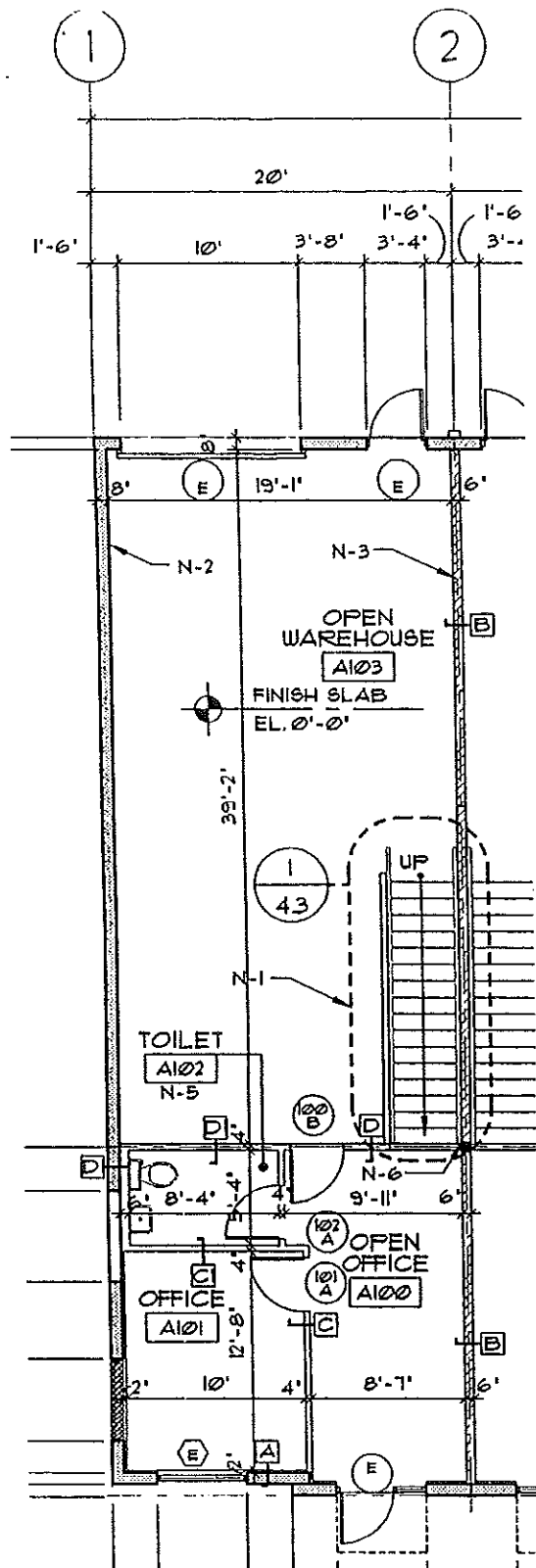
PLAN - LEVEL ONE
