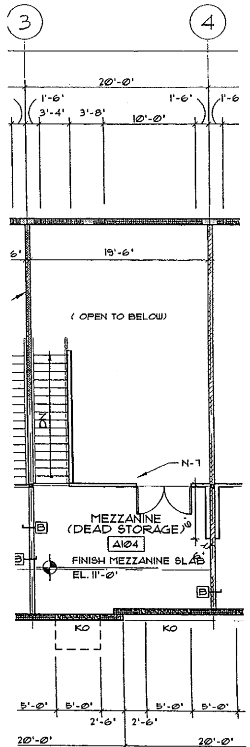
PLAN - LEVEL TWO
