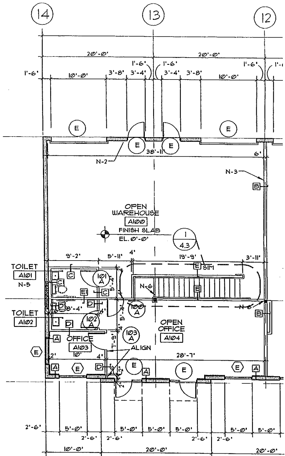
PLAN - LEVEL ONE
