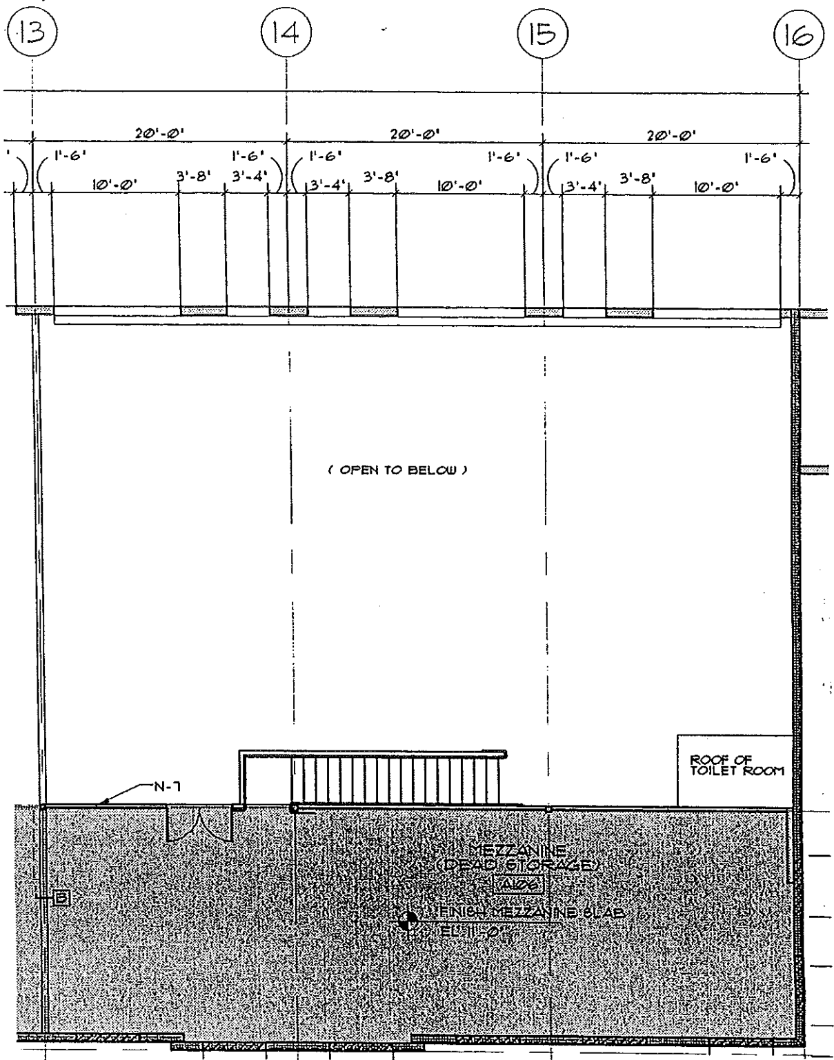
PLAN - LEVEL TWO
