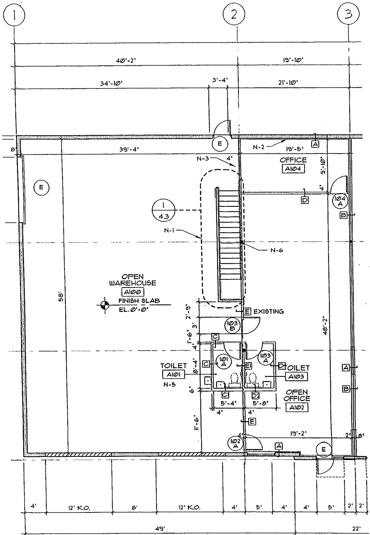
PLAN - LEVEL ONE
