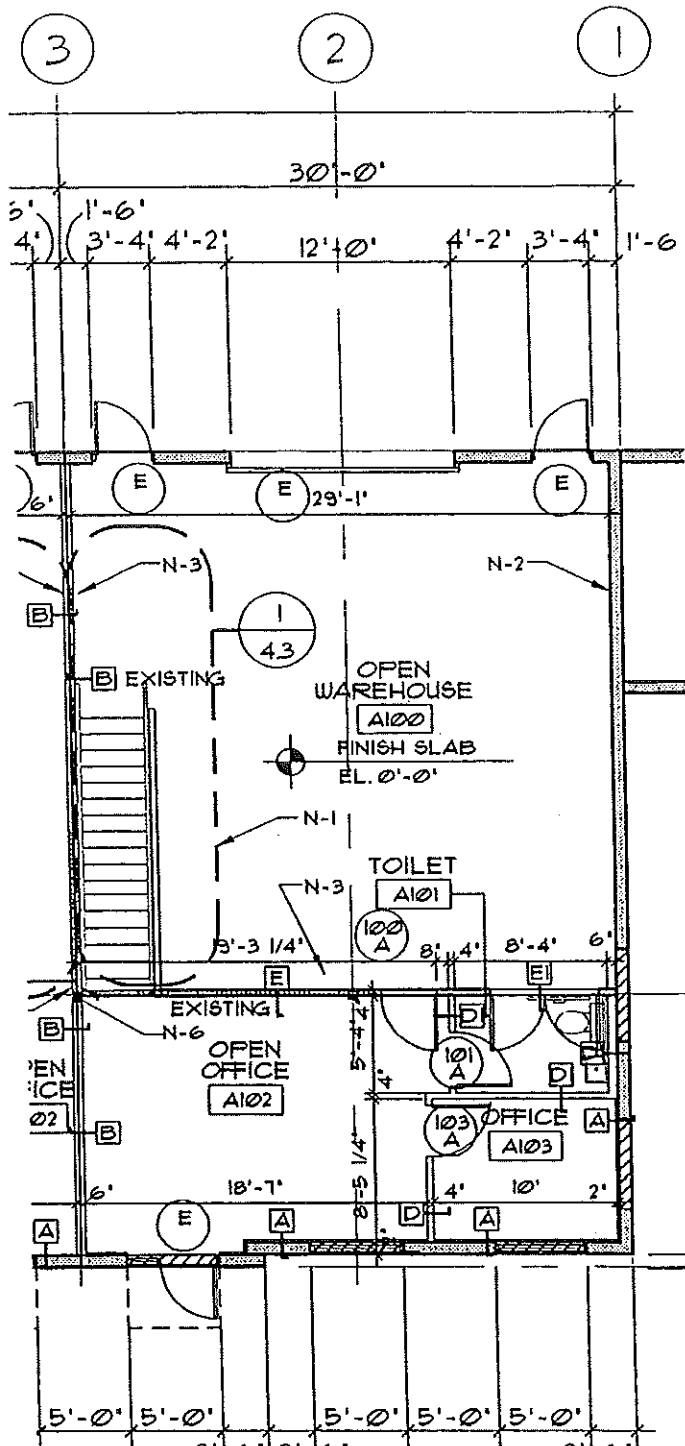
PLAN - LEVEL ONE
