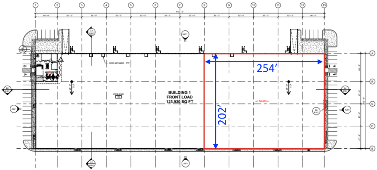
OVERALL FLOOR PLAN SCALE: 1/8" = 1'-0"
