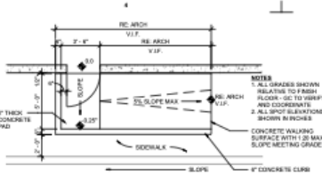
D3 CONCRETE SLOPE @ DOOR SCALE: 1/8" = 1'-0"
