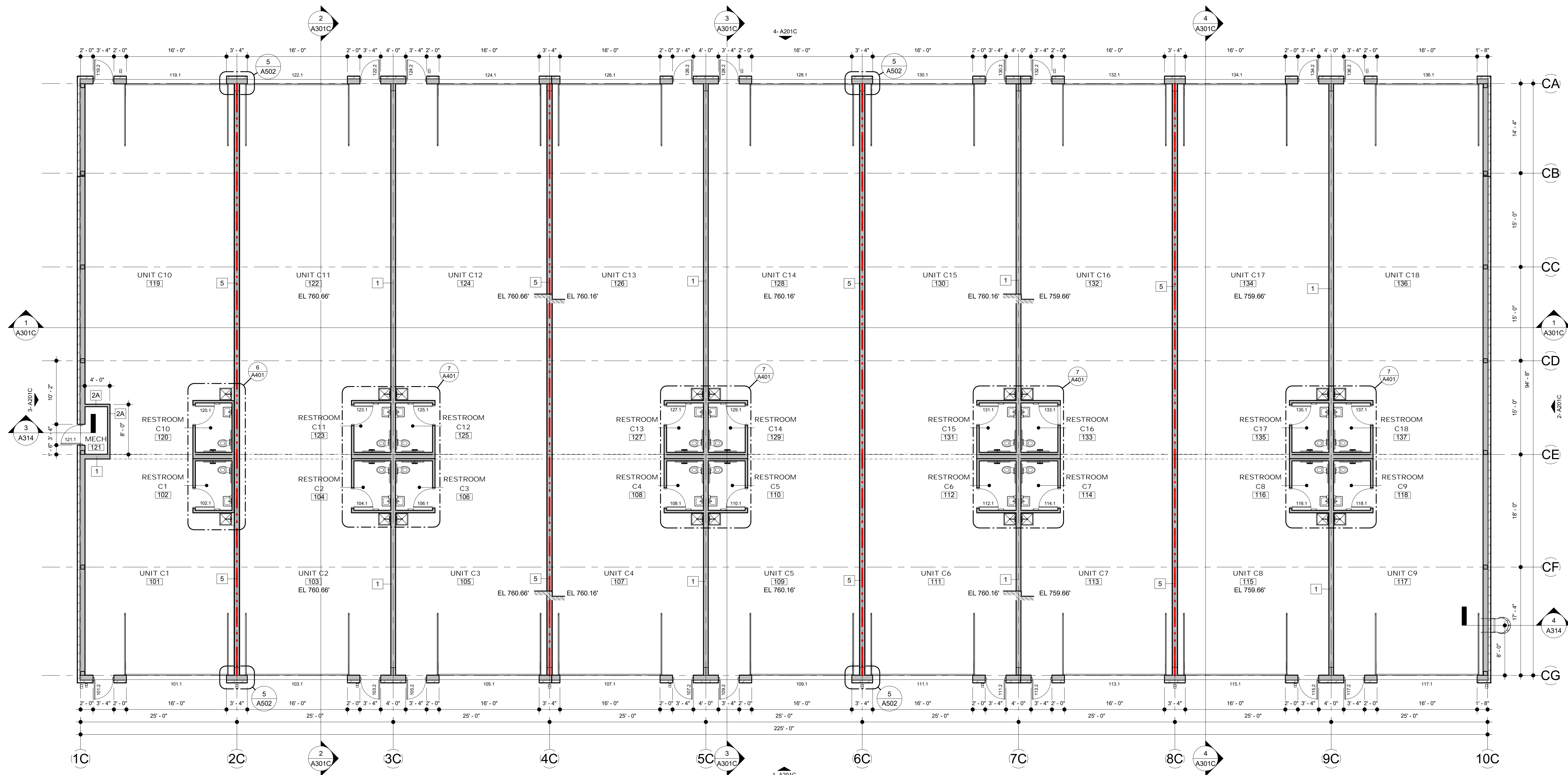
1 FIRST FLOOR PLAN - BUILDING C 1/8" = 1'-0"
