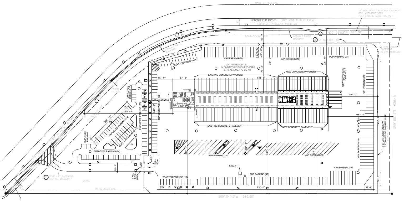
1 ARCHITECTURAL SITE LAYOUT 1" = 50'0"
