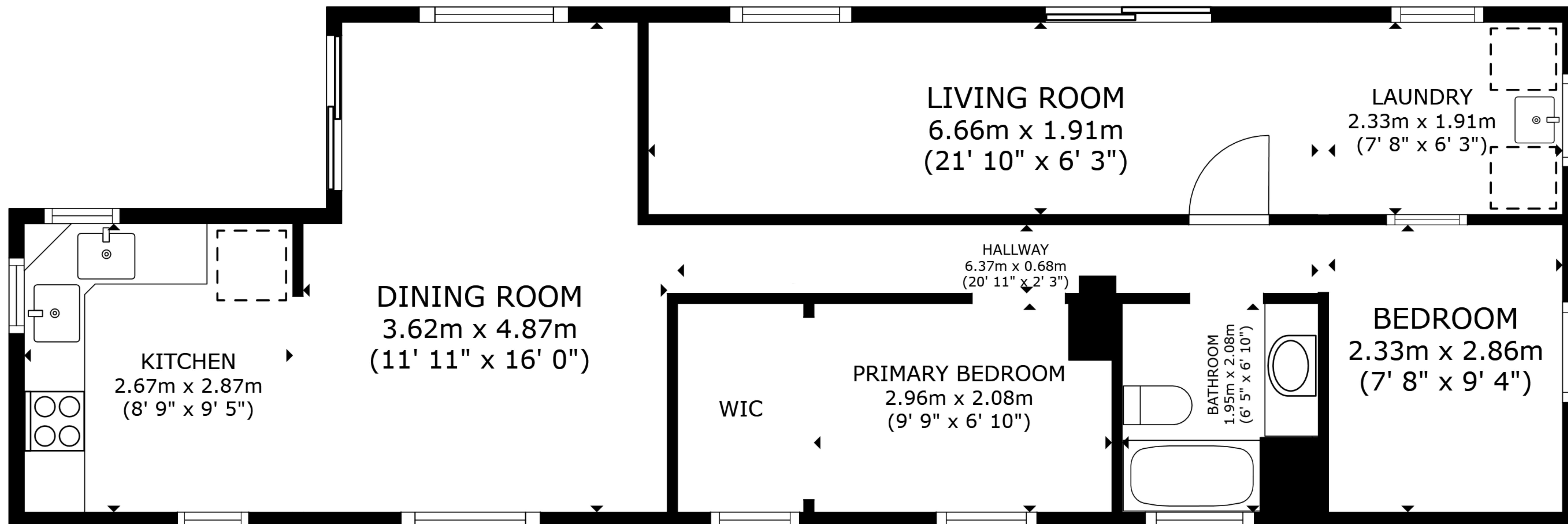
FLOOR PLAN
