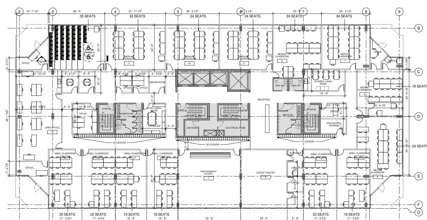
Floor Plan | Seventh Floor
