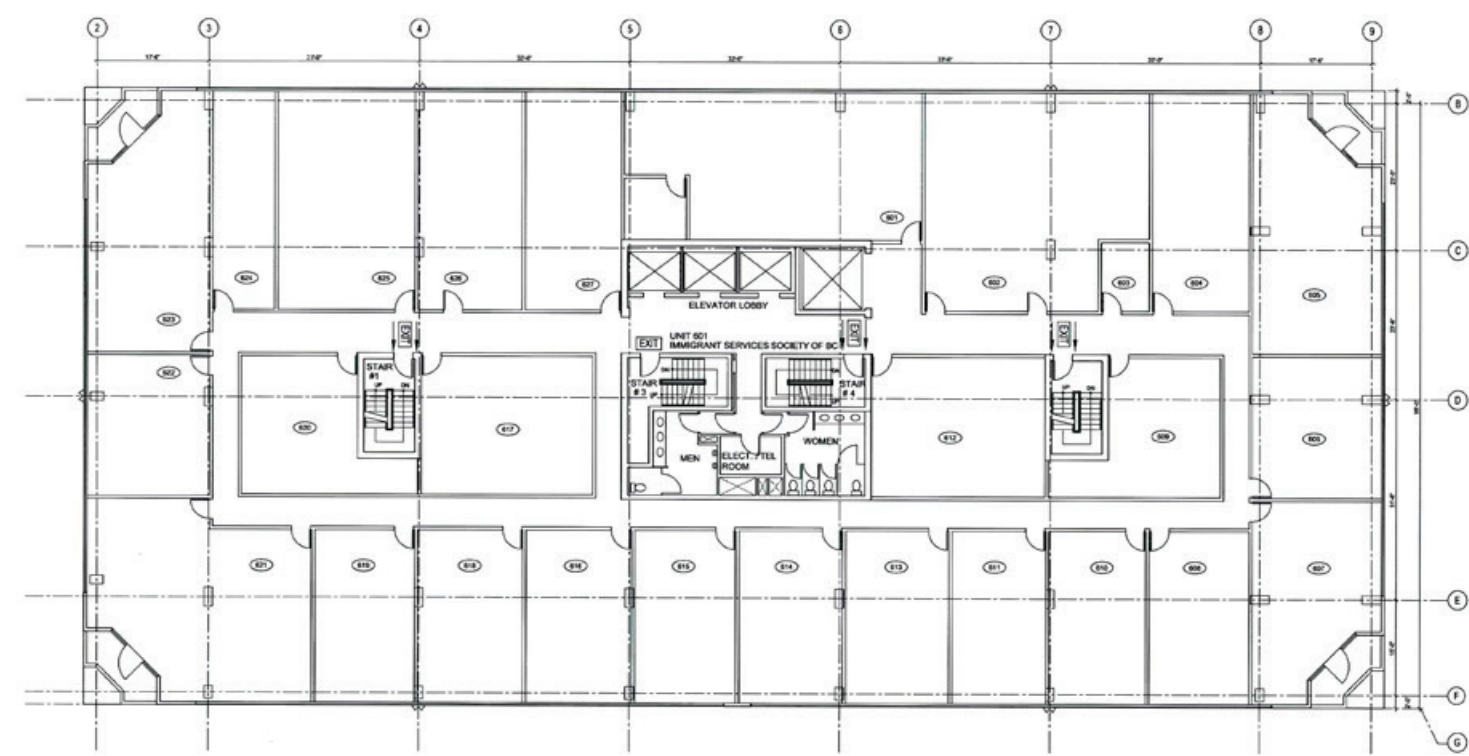
Floor Plan | Sixth Floor
