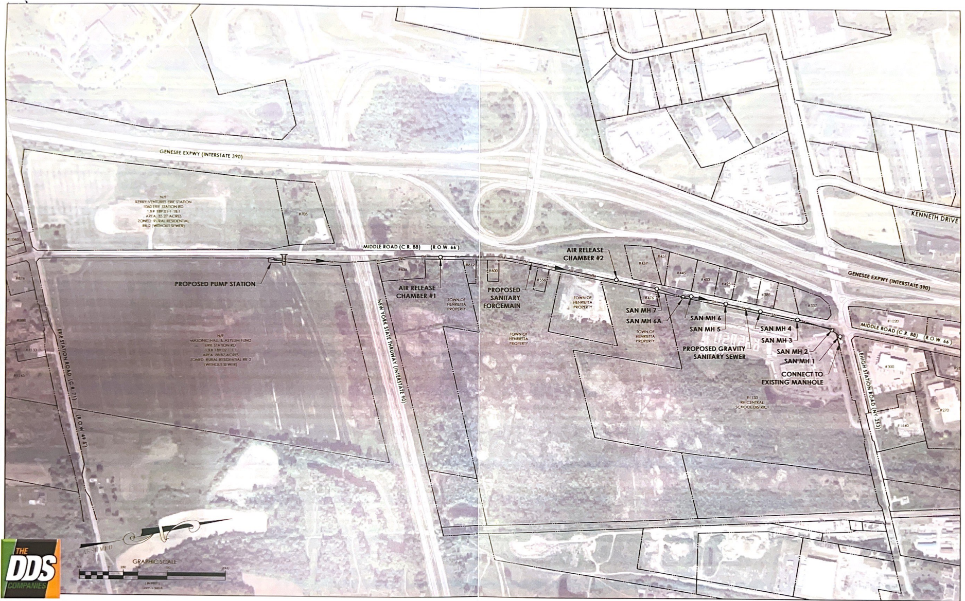
MIDDLE ROAD PUMP STATION & SANITARY SEWER OVERVIEW
