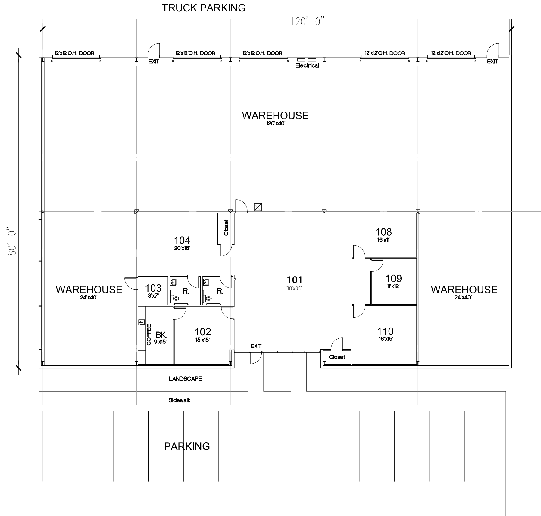
5611 GUHN RD. SUITE A3 FLOOR PLAN
