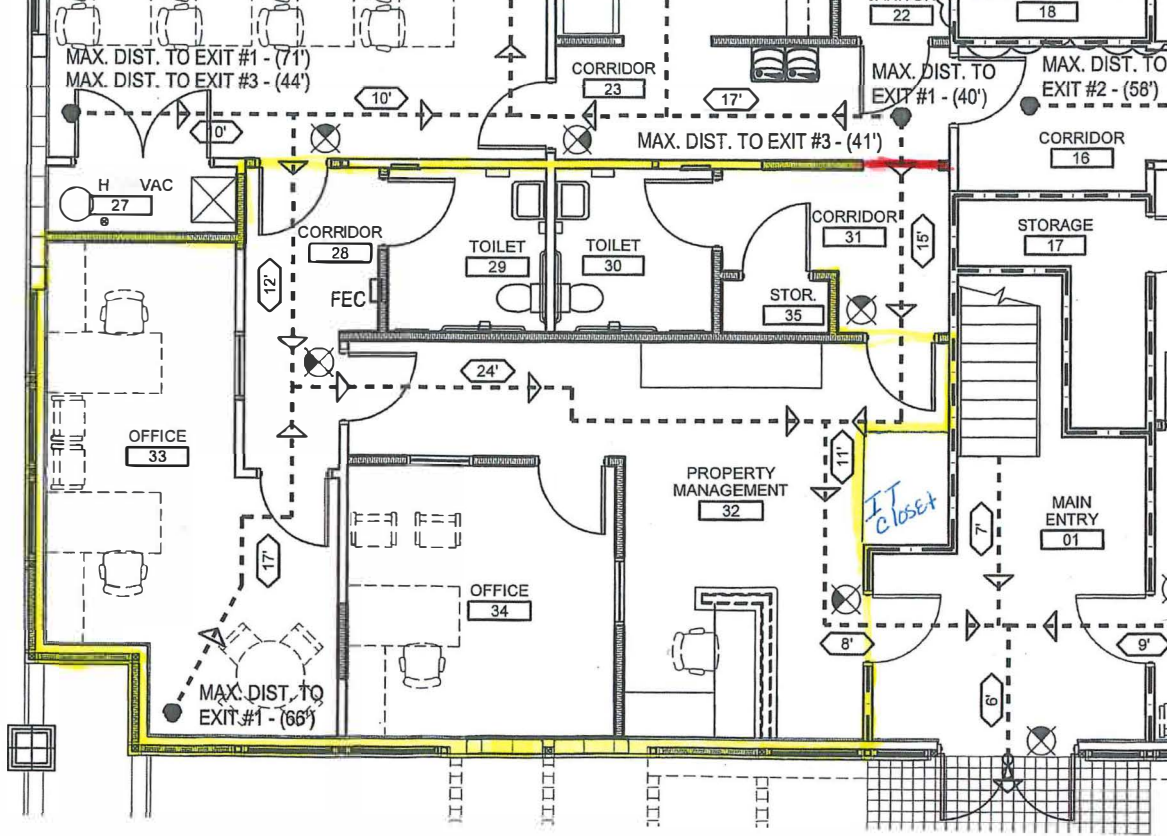
3675 20th St., Vero Beach-1st Floor Tenant Suite
