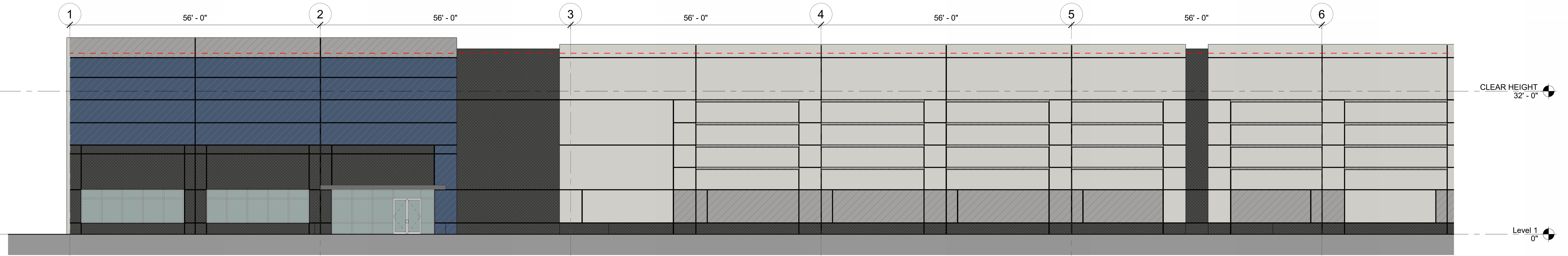
4 SOUTH ELEVATION BAYS 1-6 1" = 10'-0"
