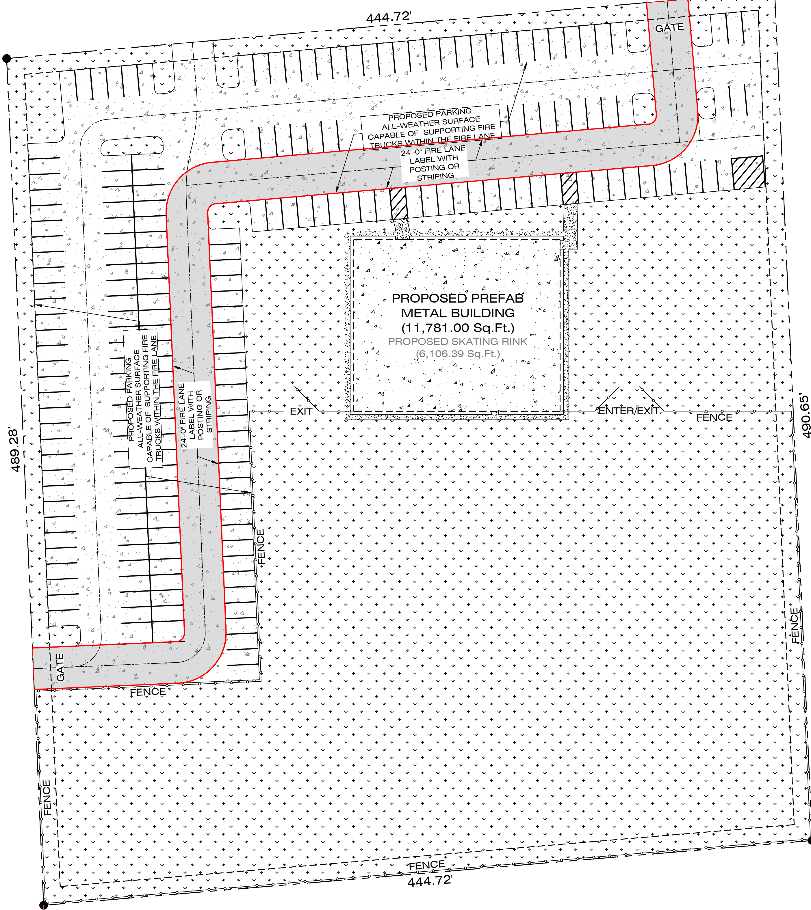
SITE LAYOUT PLAN SCALE: 1/32" = 1'-0"
