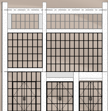
West Elevation
