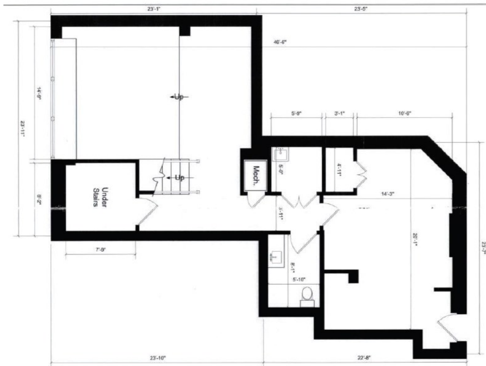
Floor Plan (Lower Level):
